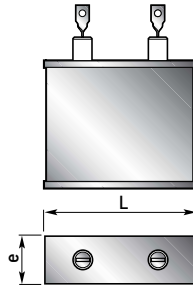
PLP 8 without mounting bracket / sans fixation
