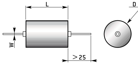
Axial leads Model TA 72
