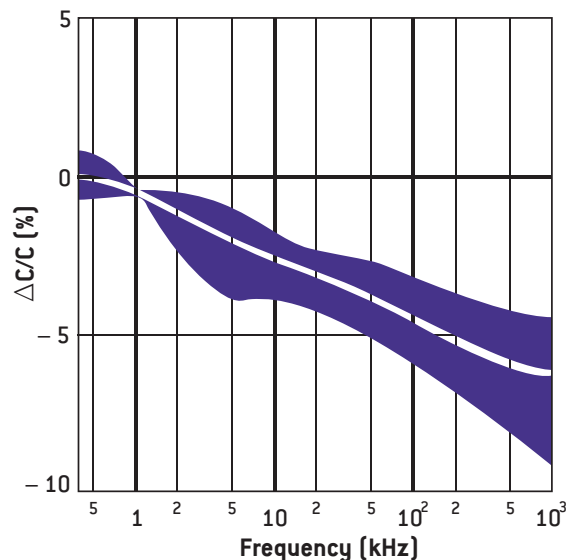
CAPACITANCE CHANGE VERSUS FREQUENCY
