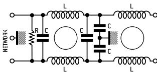
Circuit 5
