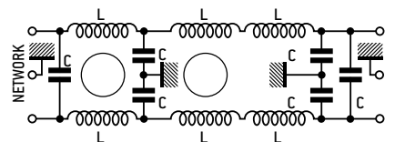
Circuit 6
