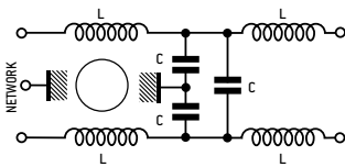
Circuit 4
