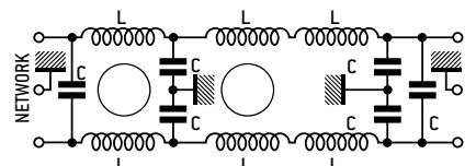
Circuit 6
