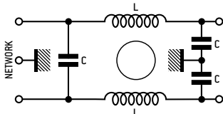
Circuit 2
