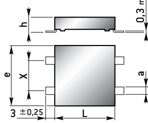
SMD leads / Sorties CMS Models/Modèles PM 90 R 1 - PM 90 SR 1 PM 90 M R 1 - PM 90 M SR 1
