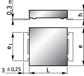
SMD leads / Sorties CMS Models/Modèles PM 90 R 2 - PM 90 SR 2 PM 90 M R 2 - PM 90 M SR 2
