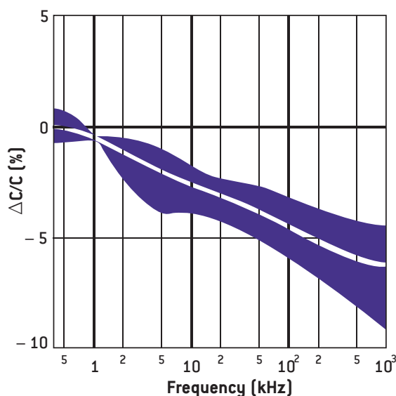
CAPACITANCE CHANGE VERSUS FREQUENCY
