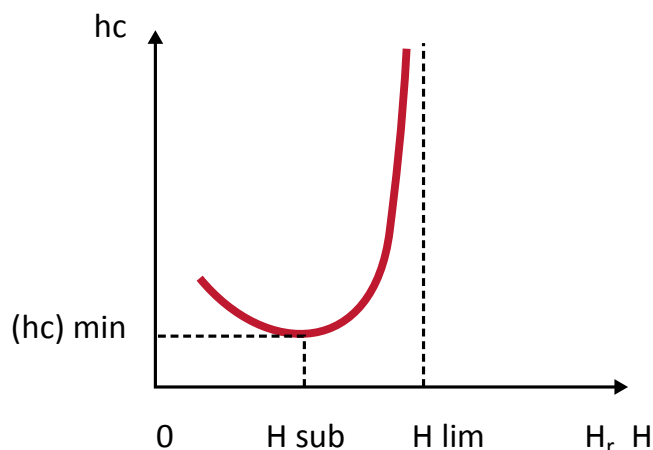
Figure 4: non-linear effect critical field h_c versus static field
